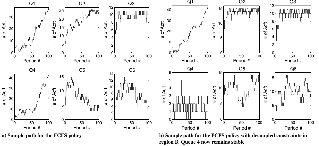
Fig. 6 Same example as in Fig. 5, but in the event of bad weather, showing the results of the FCFS and modified FCFS (decoupled constraints for region B) policies.
