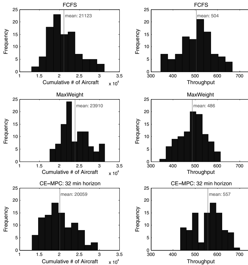
Fig. 10 Histograms of the performance results for 100 simulations, for a scenario with probabilistic forecasts as described on Fig. 9. Each simulation corresponds to an 8 h interval. On the left, we show the total cumulative number of aircraft in the system during the 8 h duration of the simulation. In other words, an aircraft is counted once for every period in which it remains in the system. On the right, we show the throughput of the policies, that is, the total number of aircraft that landed during the simulation.
