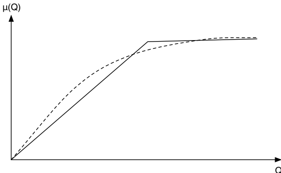
Fig. 4 Simple piecewise-linear approximation of the throughput curves used in the MPC optimization step, see Eq. (29).
