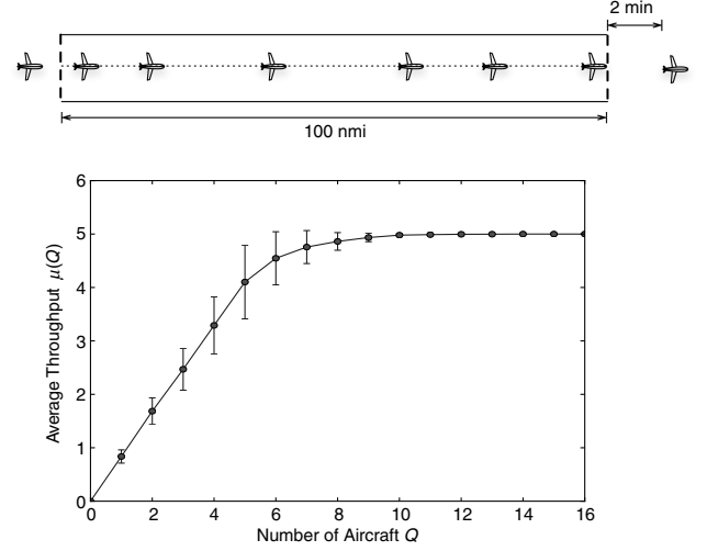
Fig. 2 Maximum throughput for the exit boundary of a simple linear control volume. The empirical curve of the mean number of departures per period was obtained via discrete-event simulation, with random arrivals. The error bars show the empirical variance of the number of departures per period. In this example, the exit boundary includes an explicit metering constraint, specifying a mandatory minimum separation of 2 min between successive aircraft.
