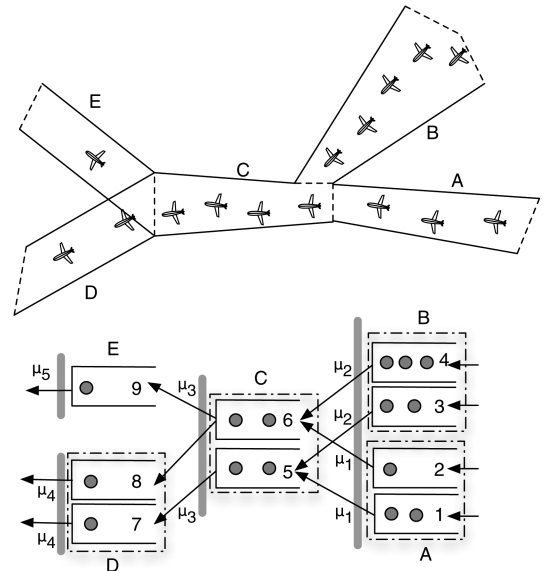
Fig. 1 Five control volumes and their corresponding abstract buffer model. The situation depicted here corresponds to two routes merging and then diverging. Each control volume except E supports two flows with distinct characteristics (e.g., different destinations, as described Sec. II.B.1), and each flow is associated with one buffer. Buffers 8 and 9 have the same flow type (destination), which allows us to include routing decisions at the output boundary of volume C . Each buffer has an associated maximum throughput function, as discussed in Sec. II.A. In this case, the buffers associated with the same control volume have the same maximum throughput function. Thick gray lines represent additional resource constraints coupling the control variables of different buffers, as described in Secs. II.B.1 and II.B.2.
