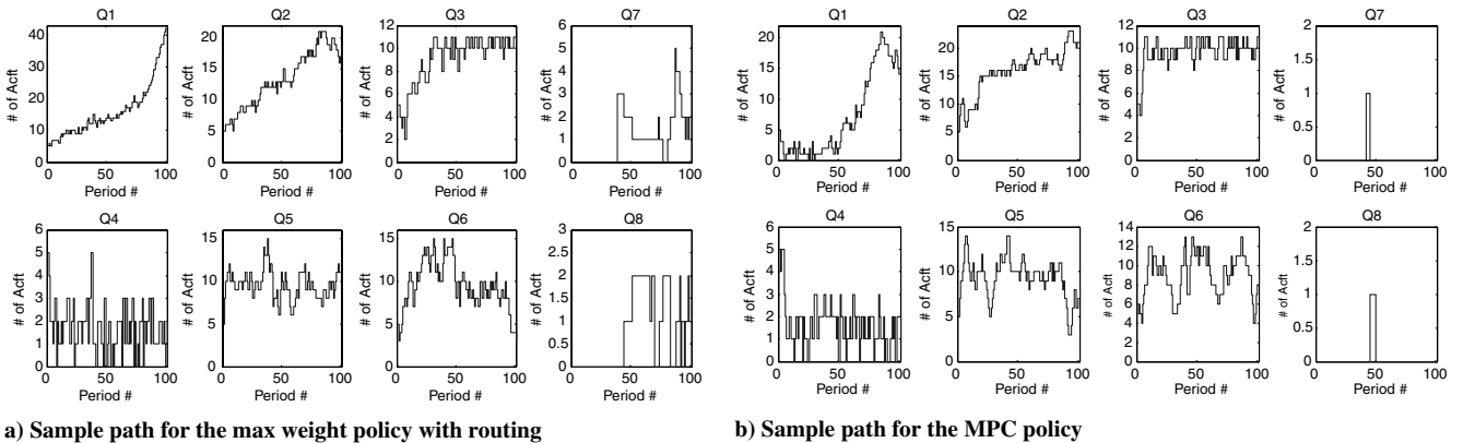
Fig. 7 Same example as in Fig. 5, but in the event of bad weather, showing the results of the MaxWeight and MPC policies.
