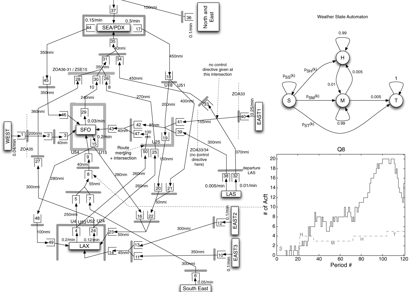
Fig. 9 Network model for TFM in the simulated system. Thick gray lines correspond to control variables coupled via the linear constraints (10) and (11). All queues start initially empty. We also show the automaton describing the probabilistic weather evolution as well as a sample trajectory of a queue in the system under the MaxWeight policy. The dashed line shows the evolution of the weather state for that sample, namely S - H - M - H - T .
