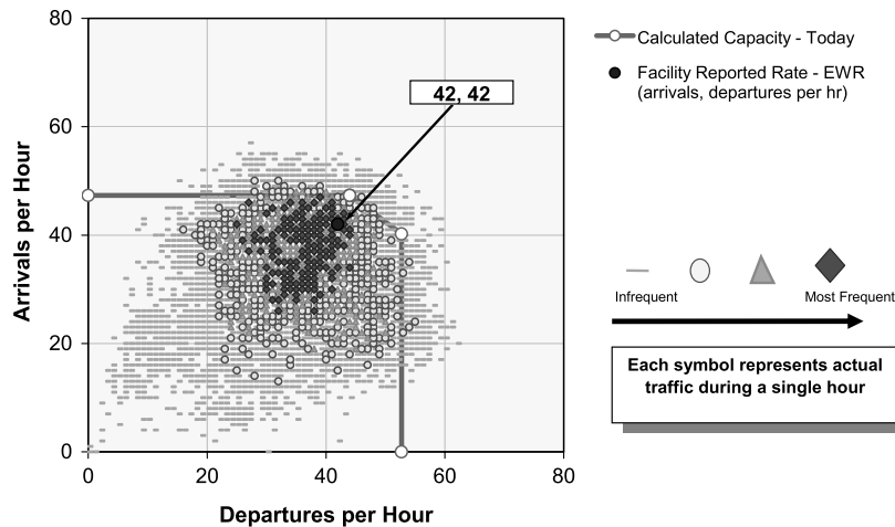
Fig. 3 Capacity envelope observed at Newark airport, under optimal conditions [28]. Any pair of arrival/departure allocation rates within the polytope is achievable. This polytope corresponds to constraints of the form (5), and depends on the airport runway configuration [26].
